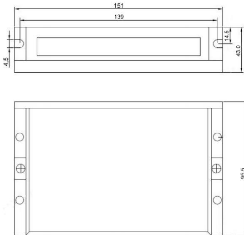
Figure 1: Mechanical specifications
