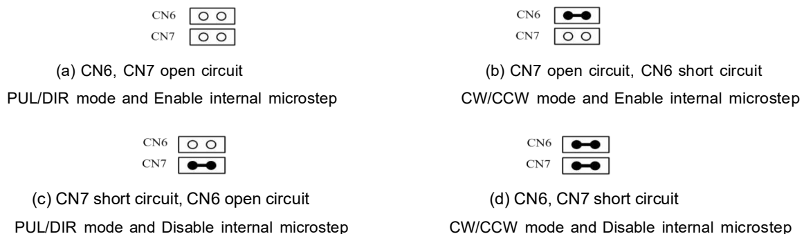
Figure 2:CN6 and CN7 jumper Settings
