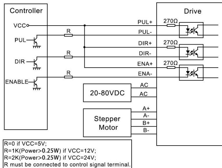
Figure 10: Typical connection
